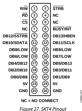
Figure 27. SKT4 Pinout
