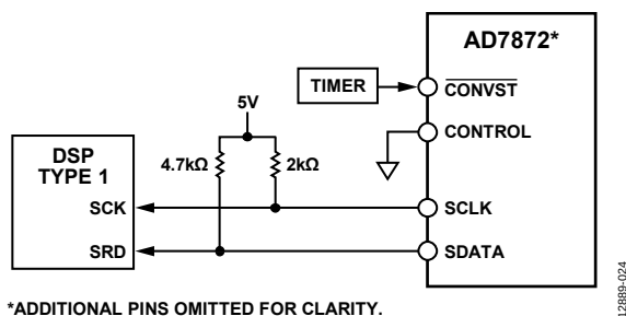
Figure 24. AD7872 to DSP Type 1 Interface
