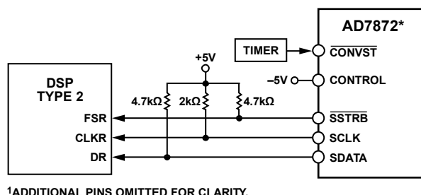
Figure 25. AD7872 to DSP Type 2 Interface
