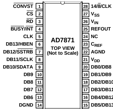
Figure 5. AD7871 DIP
