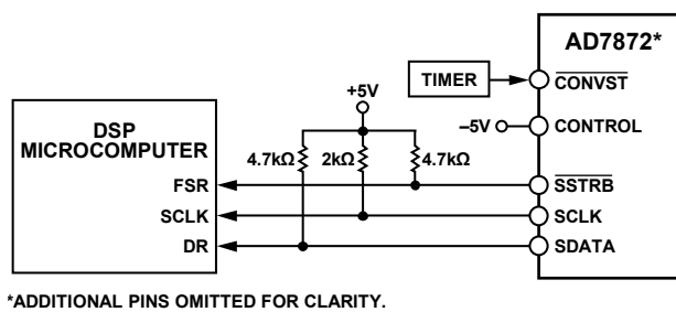
Figure 26. AD7872 to a DSP Microcomputer Serial Interface
